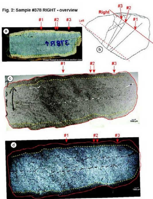
Fig. 2. As per Dr. Allaz's initial petrographic microscope observations the Flagstaff Stone shows "two distinct domains" One a fresh gray core and the other unaltered brownish rim about 1-3mm thick. Right sample.
