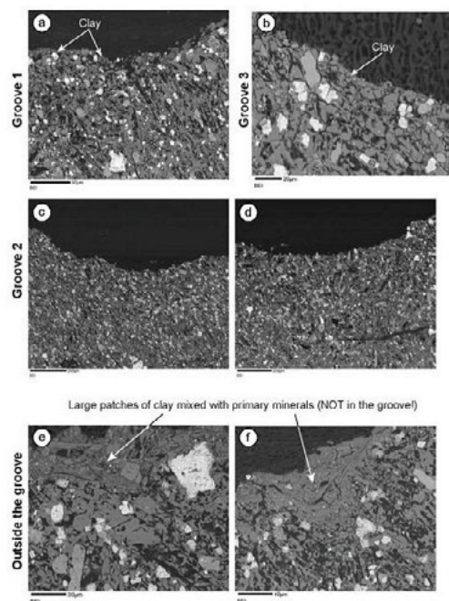
Fig. 10: Sample 378 RIGHT - BSE Images of rim domain (with clay)
